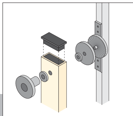
Rotative mechanism
