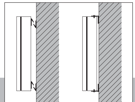
Installation system
