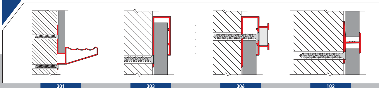
Permanent on-site installation
