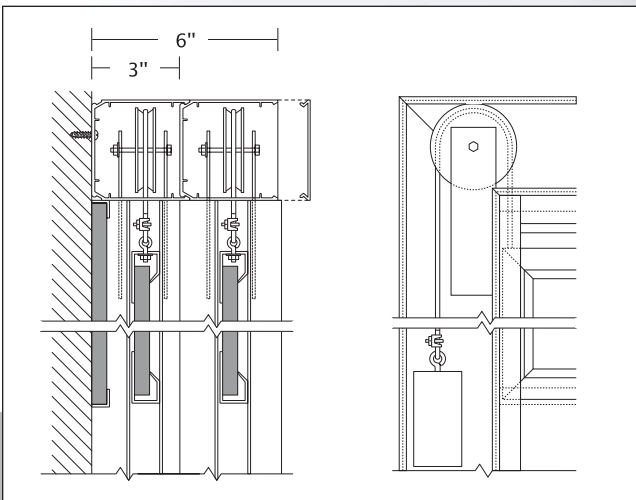
Side view of mechanism
