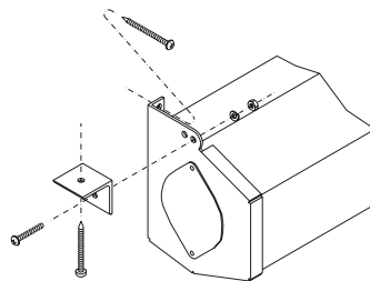
Suspended ceiling mounting
