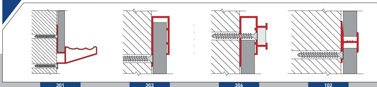
Permanent on-site installation
